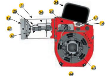
Standard Residential Oil Burner
