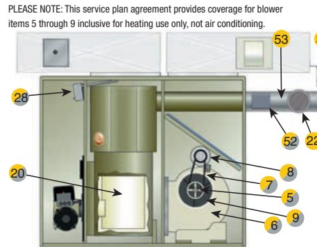
Standard Residential Warm Air Furnace
